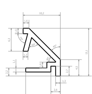
PO_05_705_A_X Aluminium
