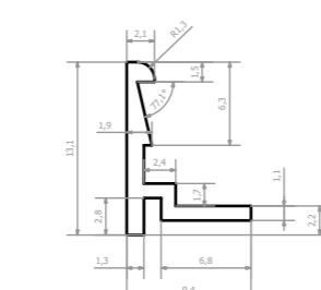
PO_05_704_A_X Aluminium
