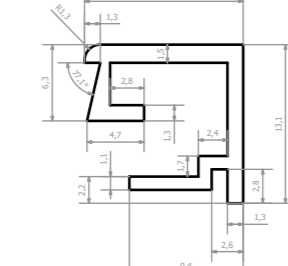
PO_05_702_A_X Aluminium
