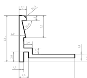
PO_05_706_A_X Aluminium
