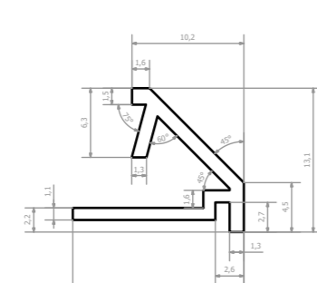
PO_05_707_A_X Aluminium
