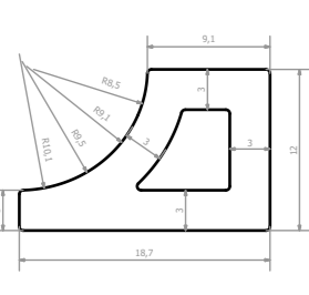
PO_05_907_A_X Aluminium
