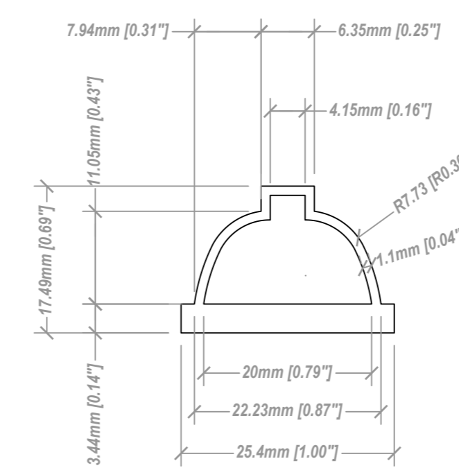
PO_04_011_A_X Aluminium
